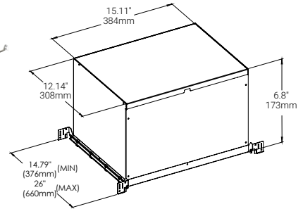
CUT HOLE: Trim & Trimless: 7 5/8" x 4 1/8"
