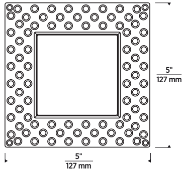
SQUARE PLASTIC (INCLUDED FOR FLANGELESS INSTALLATION)
